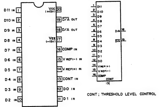
uPC648C (NEC) uPC648D (NEC) 12-BIT D/A CONVERTER WITH OPEN COLLECTOR OUTPUT — TOP VIEW —
